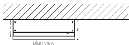
Surface Mounted - with side panels
