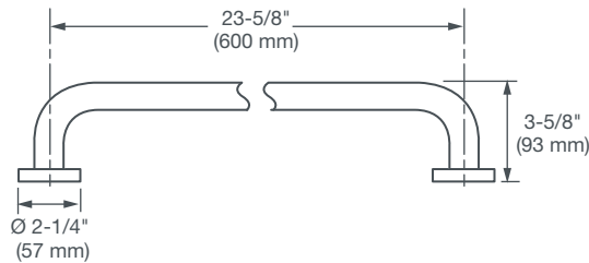
24" GRAB BAR
