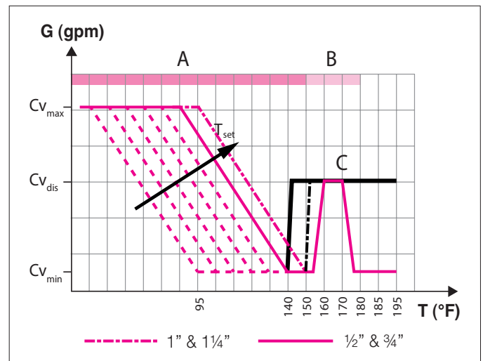
For 1162xx series with 160°F bypass temperature and 170°F closing temperature.
