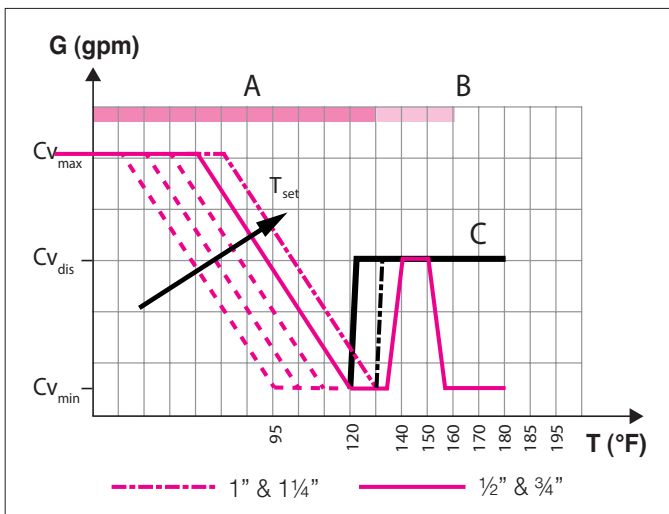
For 1166xx series with 140°F bypass temperature and 150°F closing temperature.
