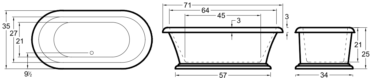
All bathtub dimensions are \pm 1/2" .
